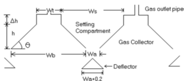
Figure 22 Details of the Gas-Liquid-Solid (GLS) Separator
